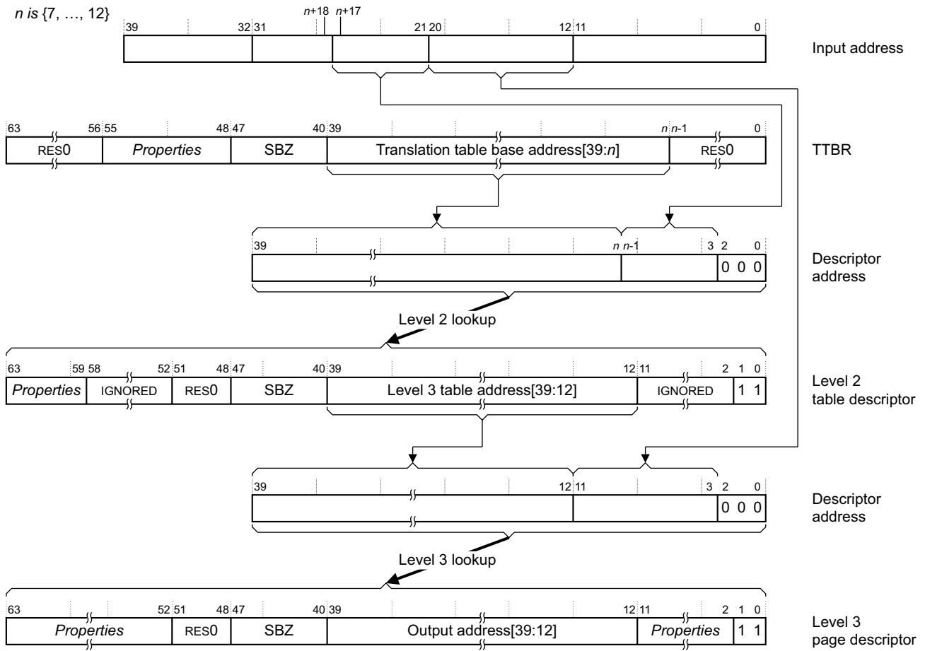
Figure K7-19 Complete VMSAv8-32 Long-descriptor format stage 1 translation, starting at level 2
