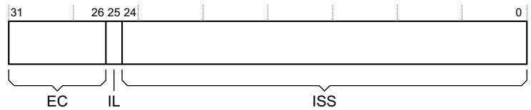
Figure G4-20 HSR format when the ISS does not include a COND field
