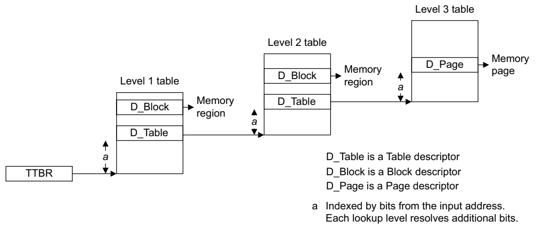
Figure D4-7 Generalized view of a stage of address translation
