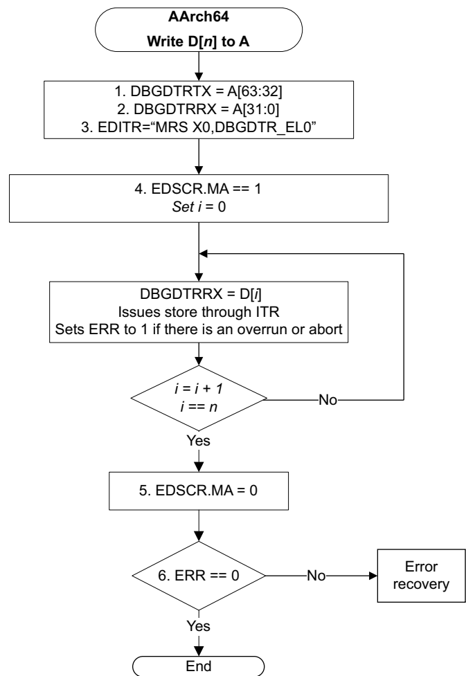
Figure K9-1 Fast code download in AArch64 (external host to target)
