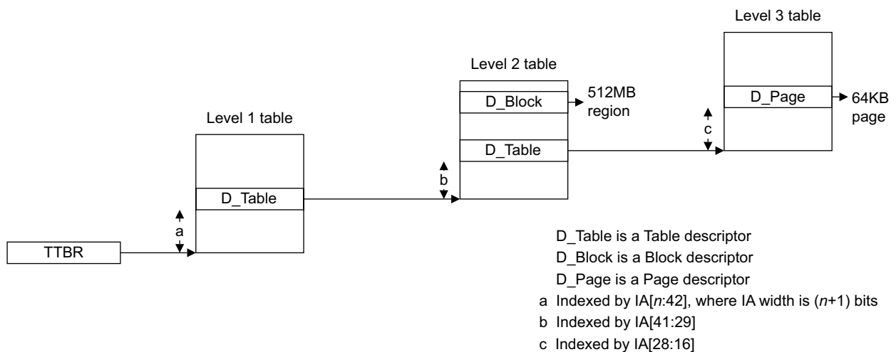
Figure D4-13 General view of VMSAv8-64 stage 1 address translation, 64KB granule
