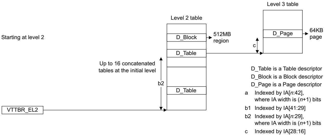
Figure D4-14 General view of VMSAv8-64 stage 2 address translation, 64KB granule
