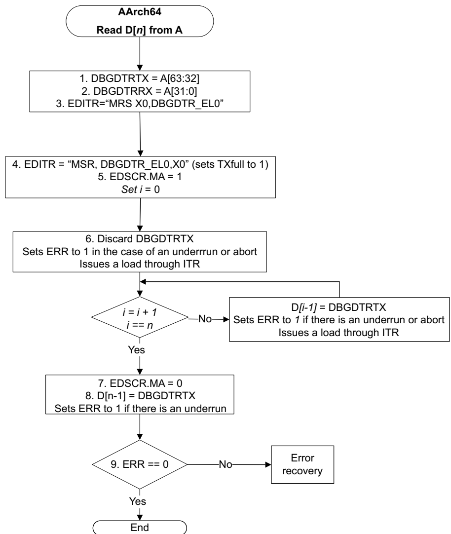
Figure K9-2 Fast data upload in AArch64 (target to external host)
