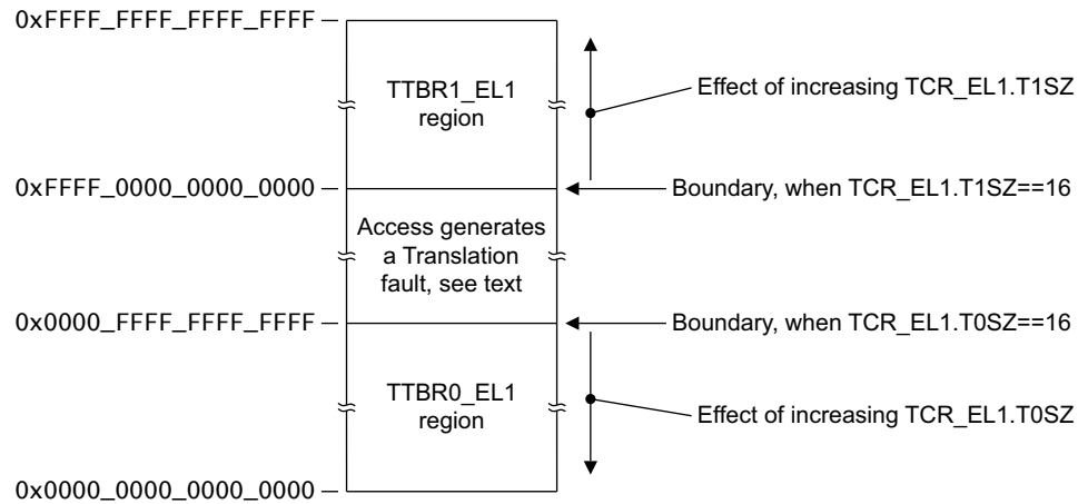
Figure D4-15 AArch64 TTBR boundaries and VA ranges
