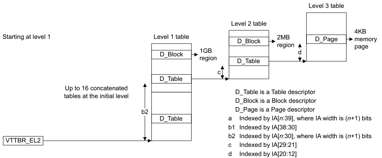
Figure D4-9 General view of VMSAv8-64 stage 2 address translation, 4KB granule
