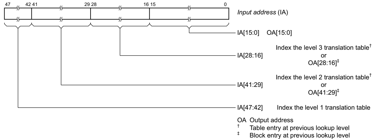
Figure D4-6 How the IA is resolved when using the 64KB translation granule
