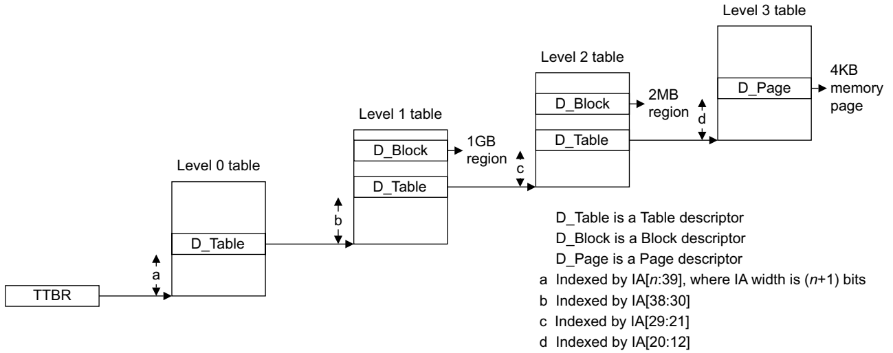
Figure D4-8 General view of VMSAv8-64 stage 1 address translation, 4KB granule
