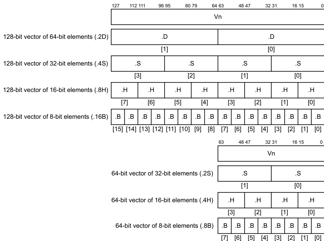
Figure A1-1 SIMD vectors in AArch64 state
