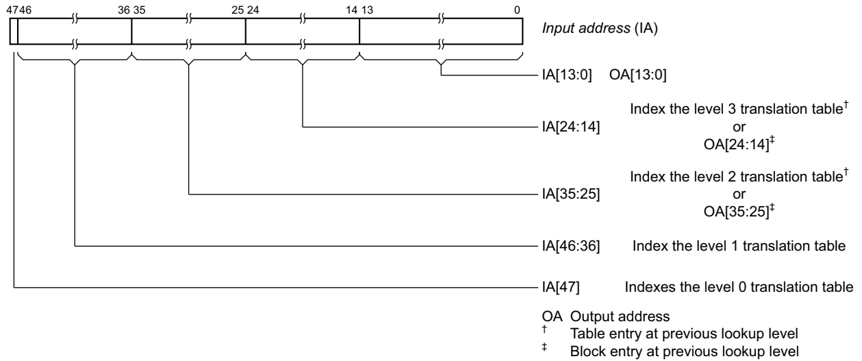
Figure D4-5 How the IA is resolved when using the 16KB translation granule
