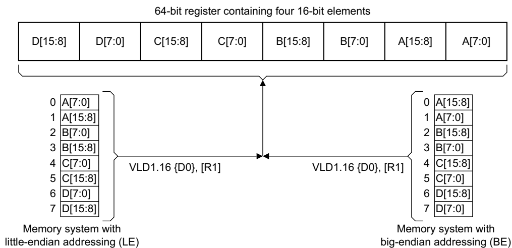
Figure E2-3 Advanced SIMD byte order example for AArch32
