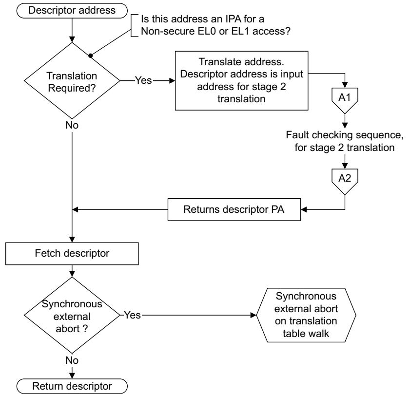
Figure D4-18 Fetching the descriptor in a VMSAv8-64 translation table walk
