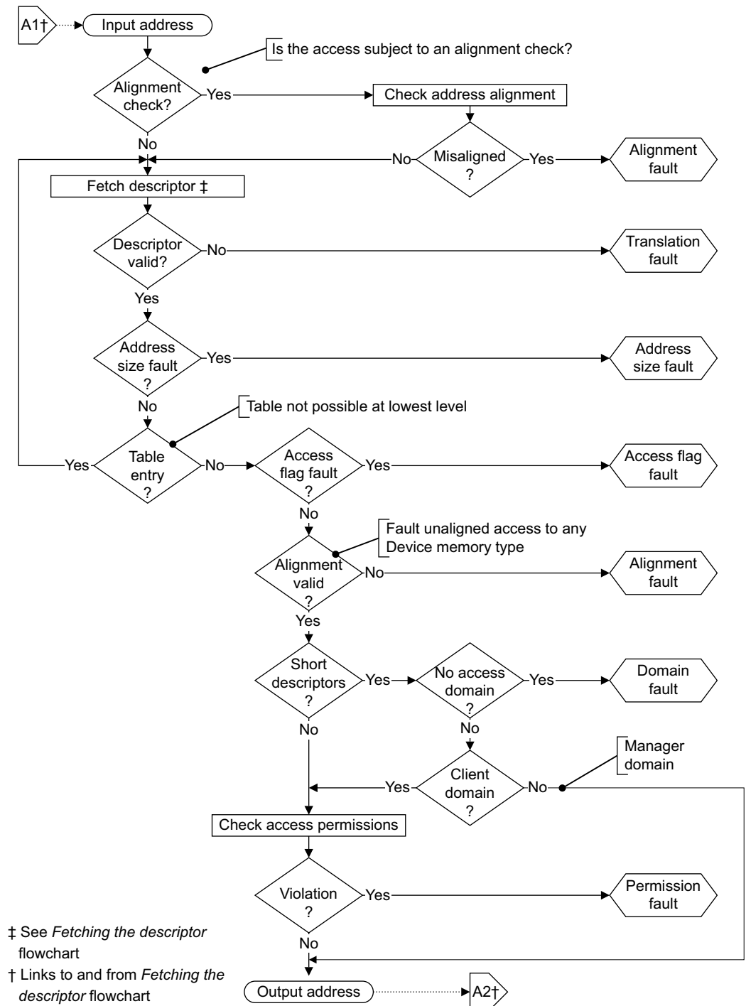
Figure G4-18 VMSAv8-32 fault checking sequence
