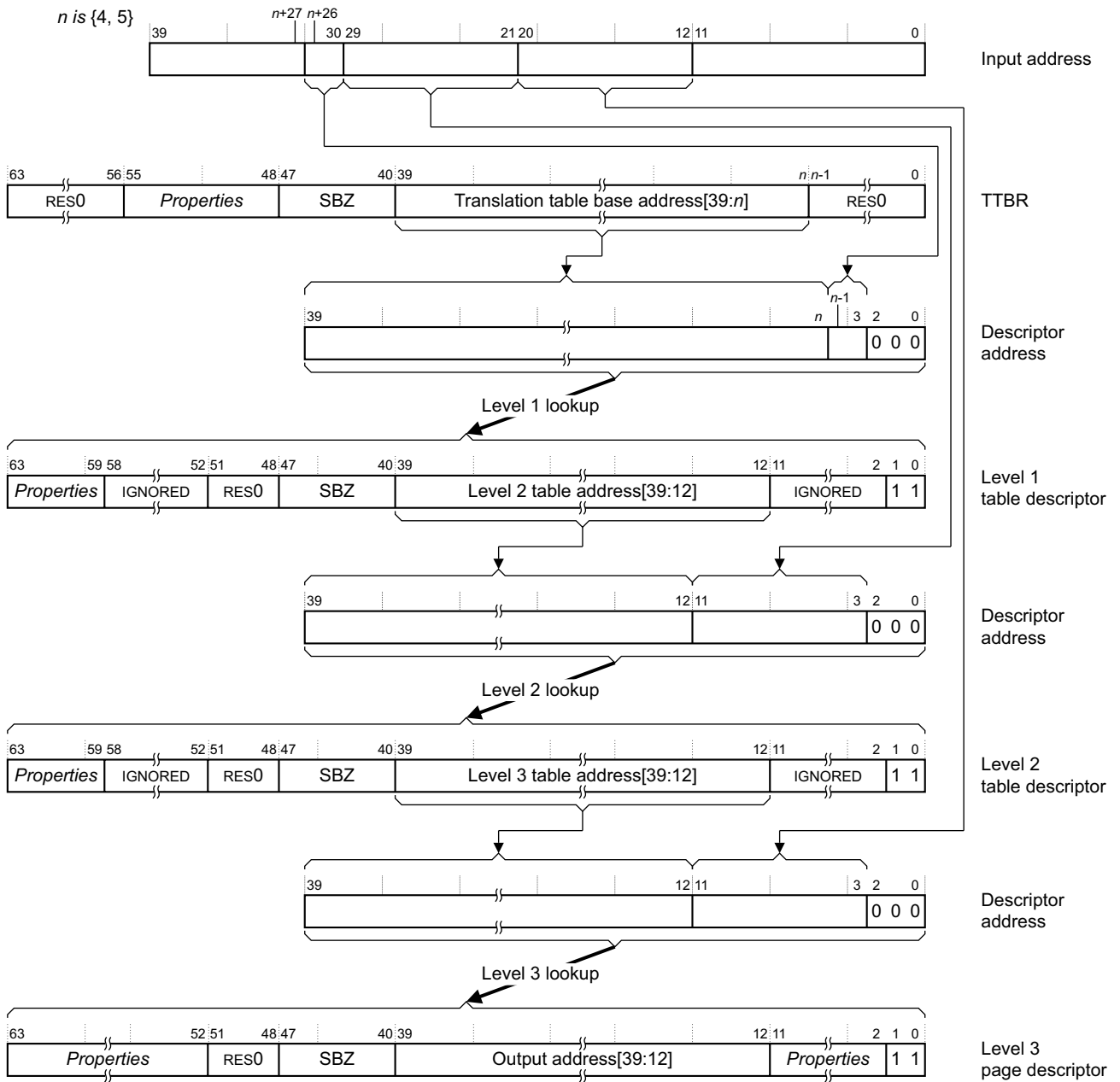
Figure K7-18 Complete VMSAv8-32 Long-descriptor format stage 1 translation, starting at level 1
