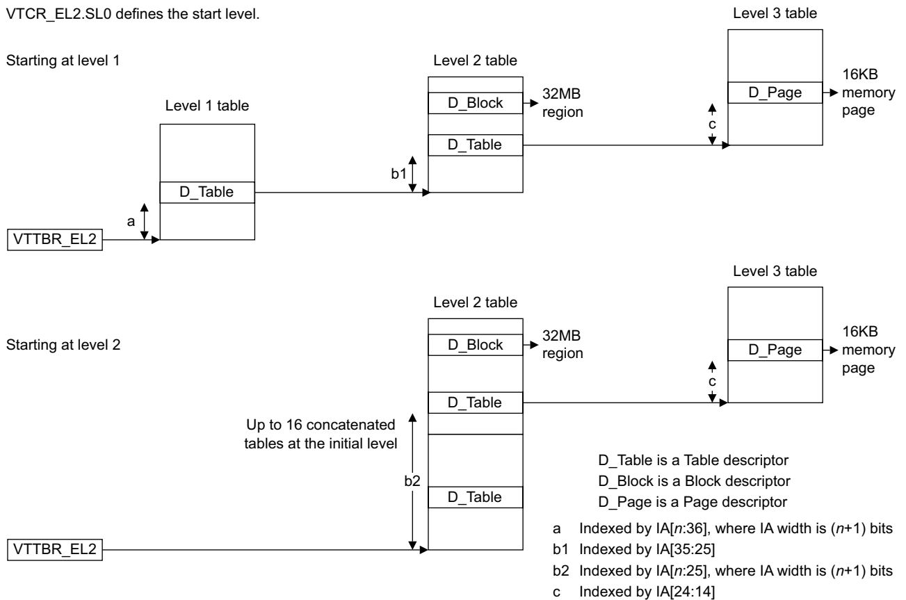
Figure D4-12 General view of VMSAv8-64 stage 2 address translation, 16KB granule
