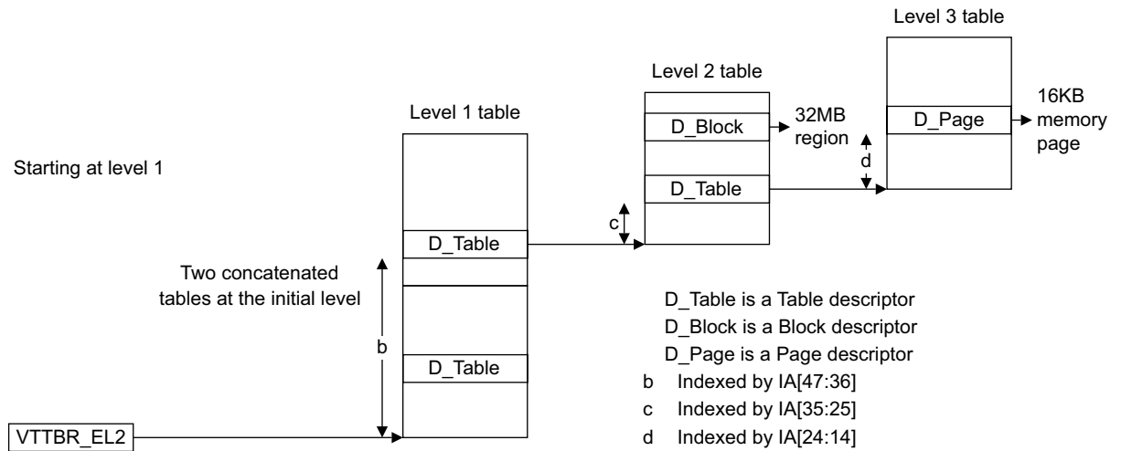
Figure D4-11 VMSAv8-64 stage 2 address translation, 16KB granule, 48 bit input address
