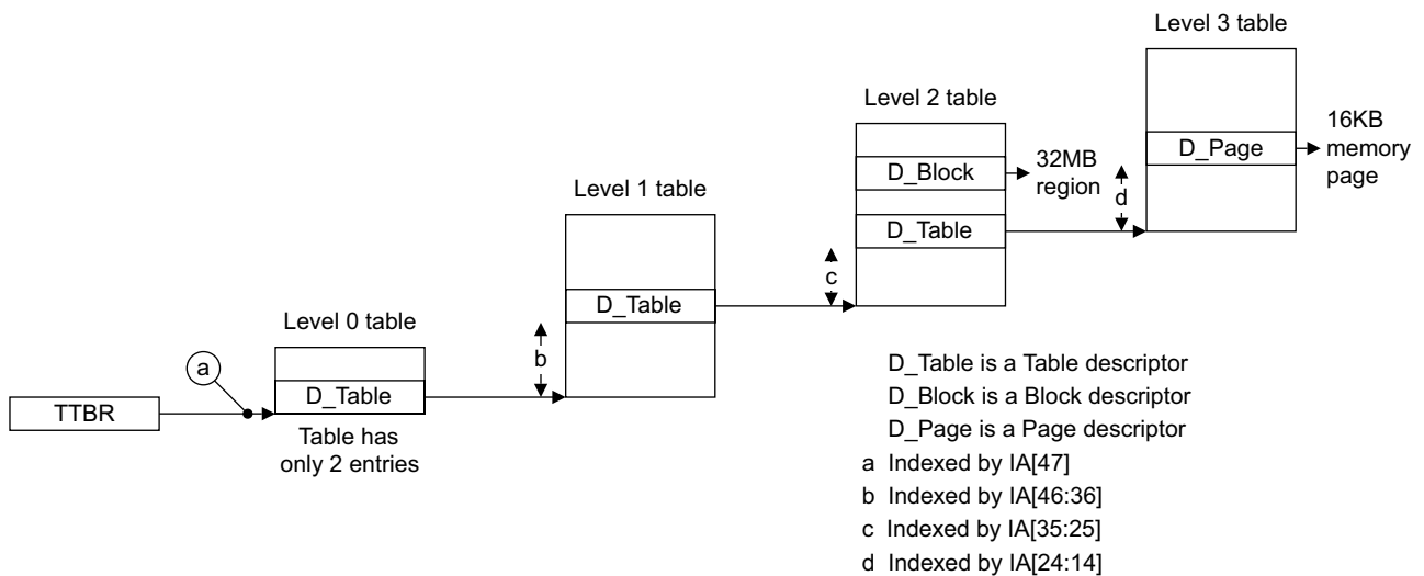
Figure D4-10 General view of VMSAv8-64 stage 1 address translation, 16KB granule
