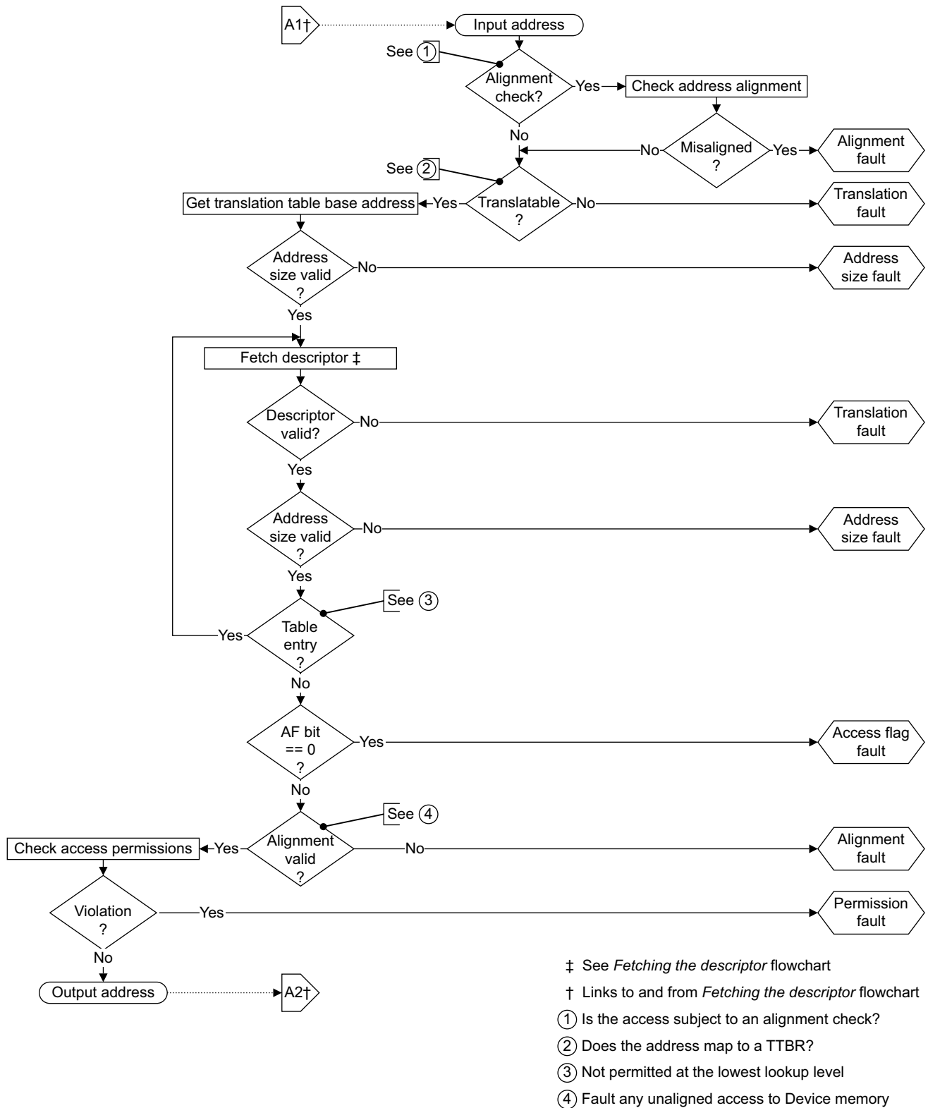
Figure D4-19 VMSAv8-64 fault checking sequence
